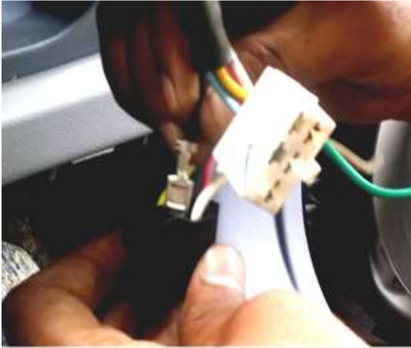
Ignition Pin from Car Current Socket (near Key) be pull out & inserted in Place of 87 Wire in Relay Socket of MVT 300.
