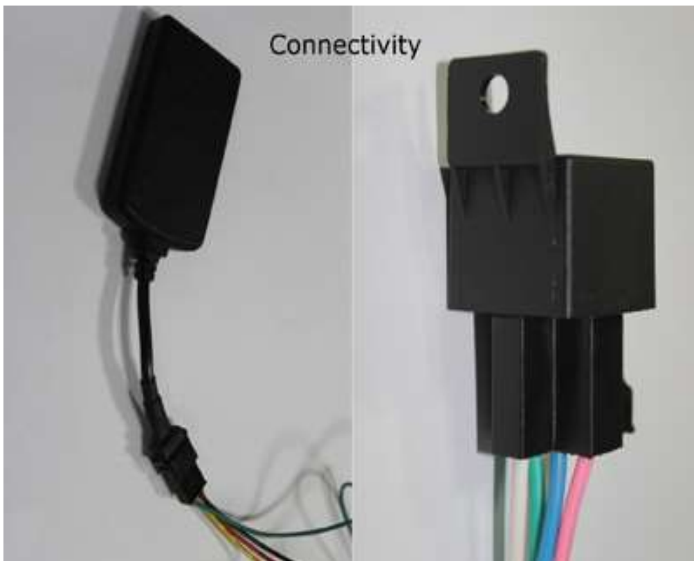
Ignition Pin from Car Current Socket (near Key) be pull out & inserted in Place of 87 Wire in Relay Socket of MVT 300.
